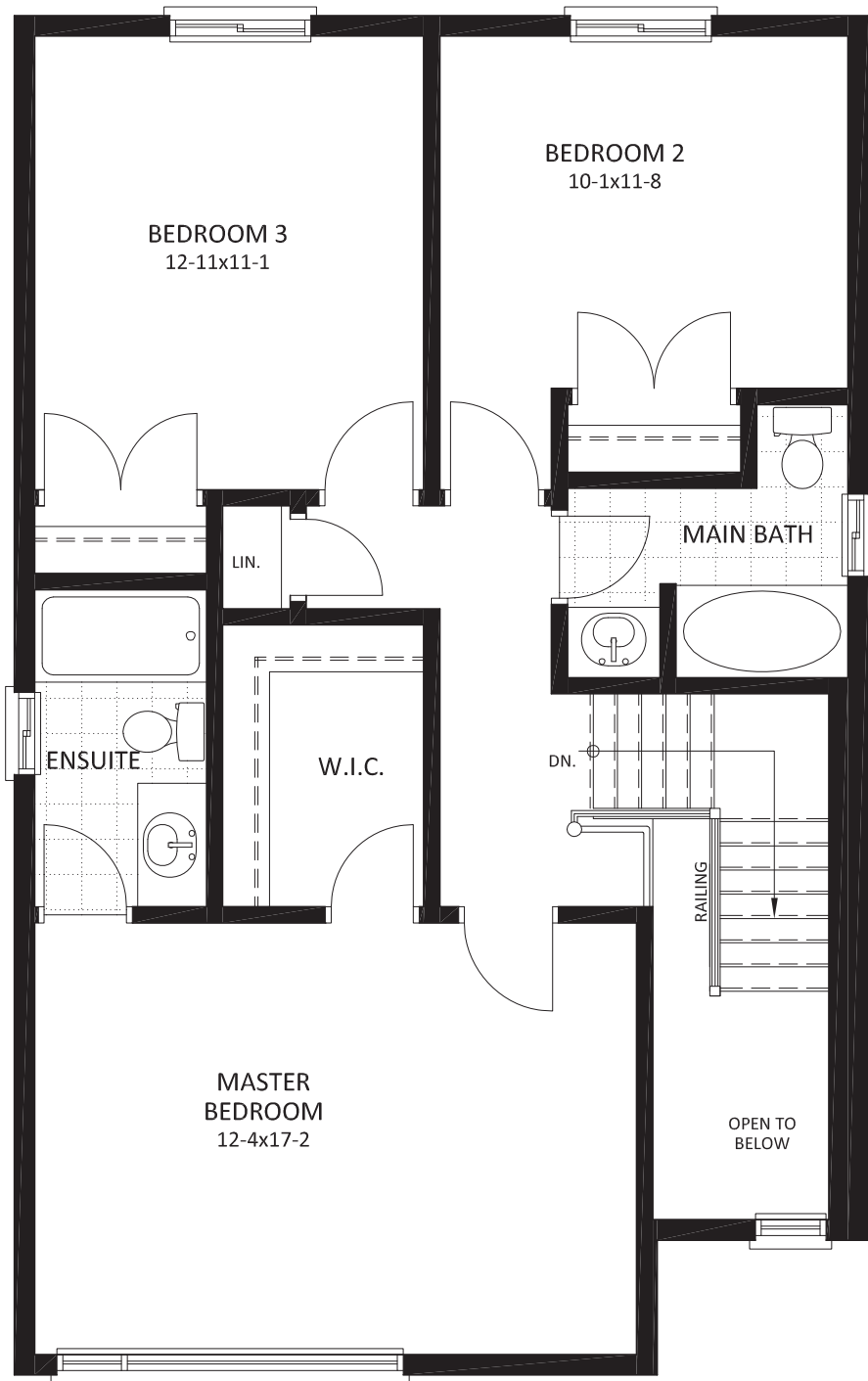
THE SELDON SECOND FLOOR PLAN 'A'
