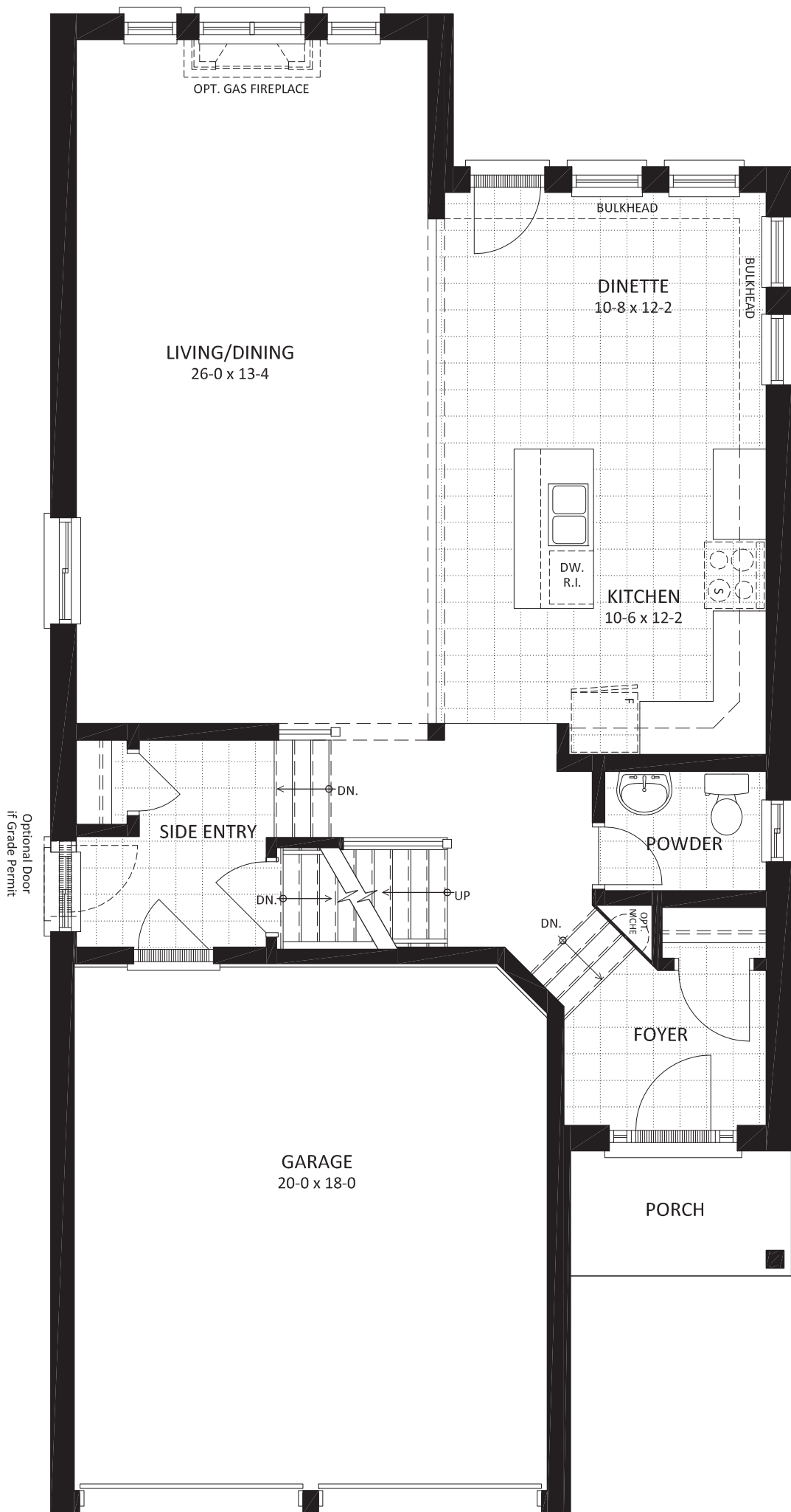
THE MORTON MAIN FLOOR PLAN 'A'
