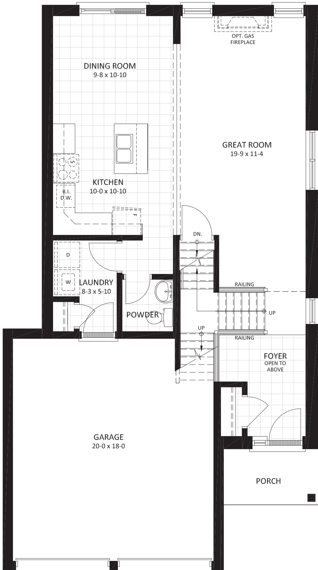
THE STANWICK MAIN FLOOR PLAN 'A'
