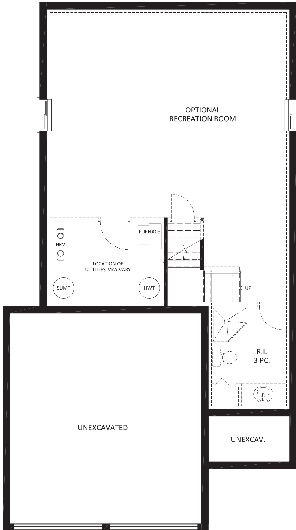
THE STANWICK BASEMENT FLOOR PLAN 'A' & 'B'
