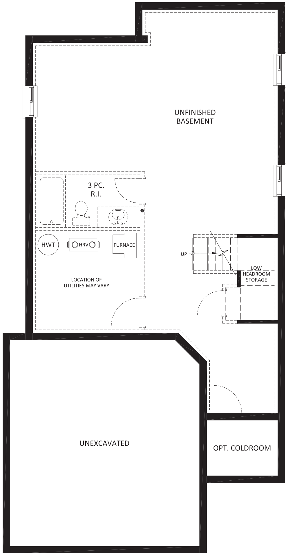
THE TILTON BASEMENT FLOOR PLAN
