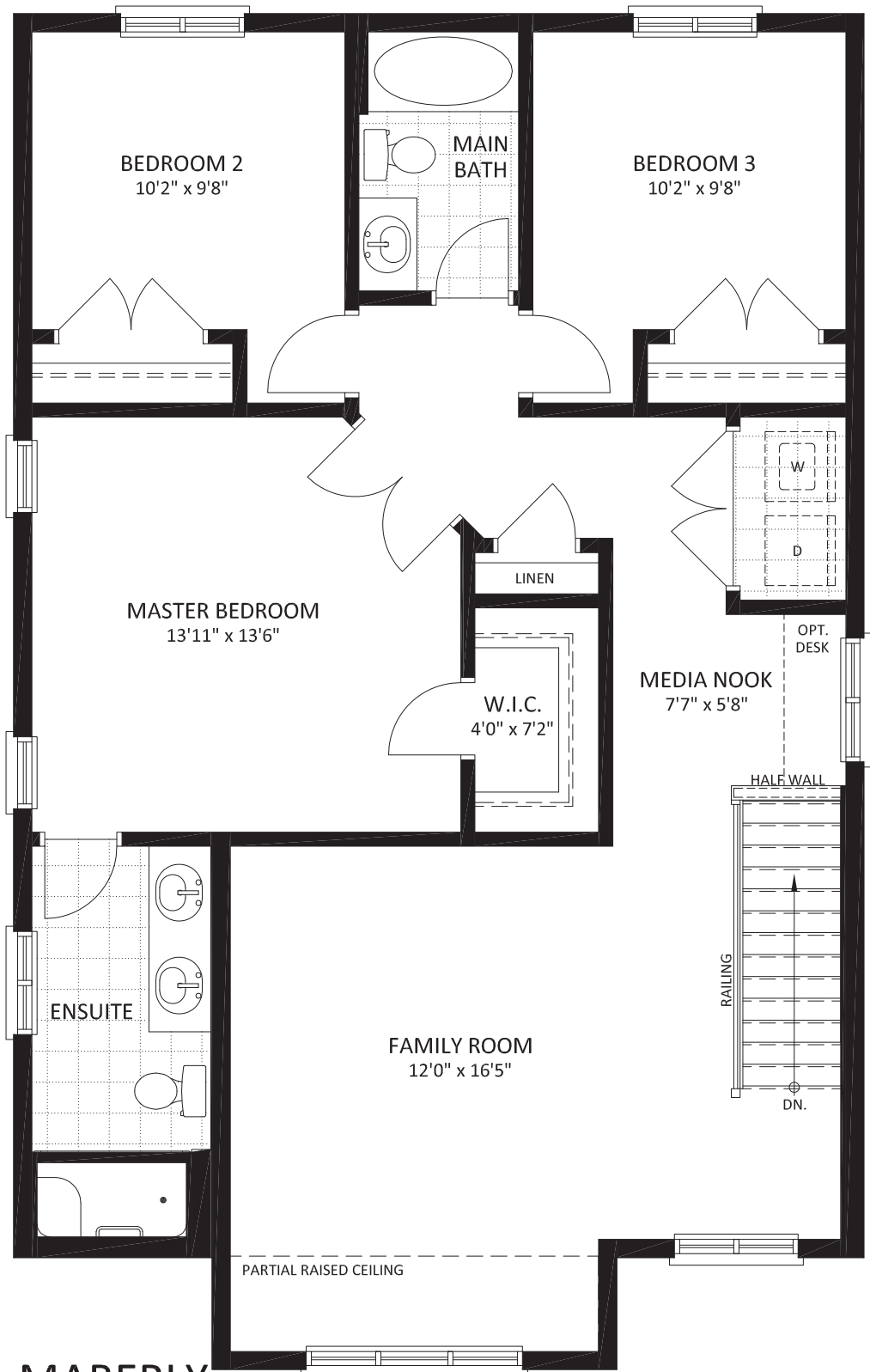
MABERLY SECOND FLOOR PLAN FAMILY ROOM LAYOUT
