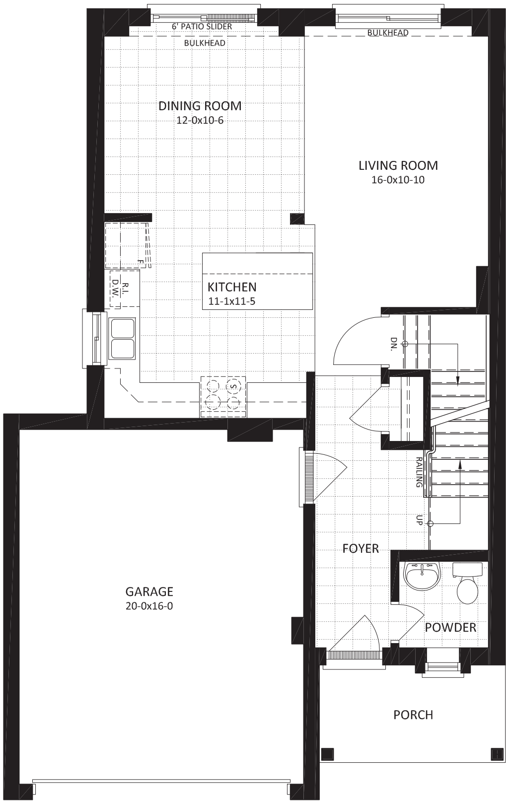
HE NEWBOLD MAIN FLOOR PLAN 'A' & 'B'
