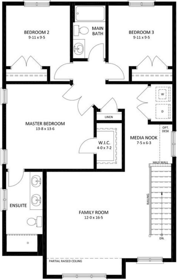
SECOND FLOOR PLAN 3 BEDROOM 1102 SQ.FT.
