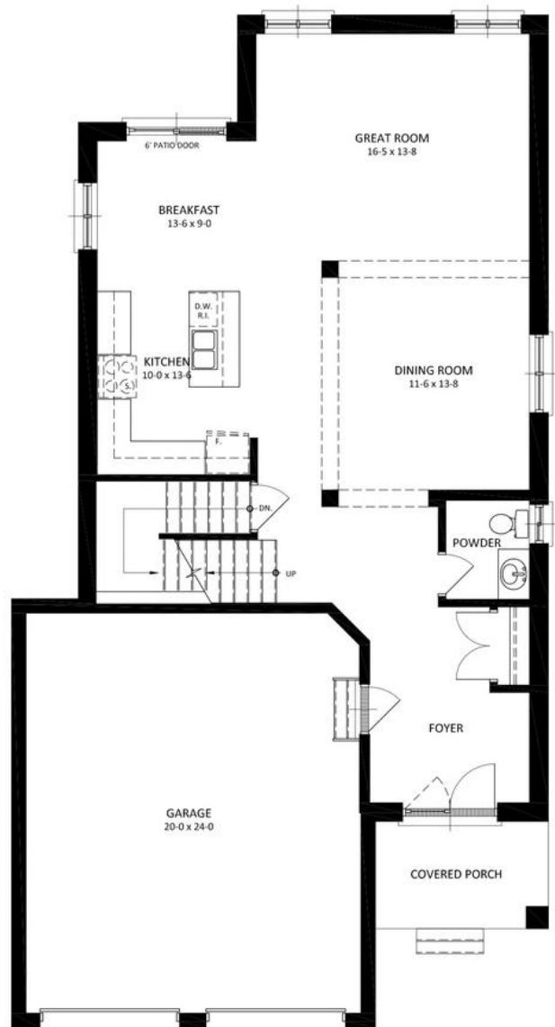
MAIN FLOOR PLAN 1069 SQ.FT.
