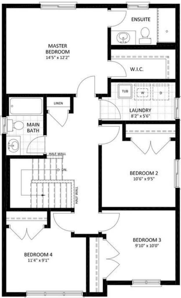
SECOND FLOOR PLAN 935 SQ.FT.
