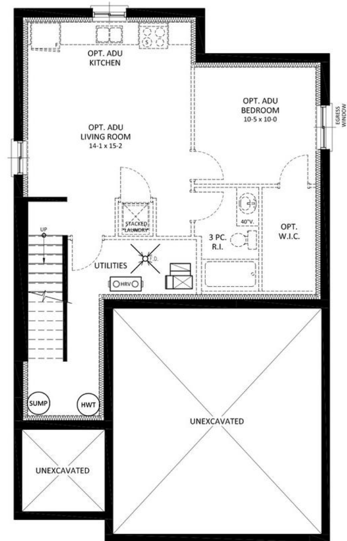
FOUNDATION PLAN
